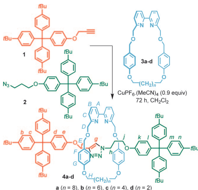
Scheme 1. Variation of macrocycle size in the bipyridine-mediated CuAAC-AT reaction.
