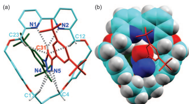
Figure 3. Single-crystal X-ray structure [14] of [2]rotaxane 6 viewed along the thread axis a) in capped sticks representation with selected close contacts indicated (majority of H atoms omitted for clarity) and b) in partial space-fill representation. Selected bond lengths (in Å): N1–H31 2.57, N2–H31 2.49, C31–H23 2.99, C31–H12 2.80, N4–H1 2.65, N4–H4 2.48, N5–H1 2.84, N5–H4 2.65.
