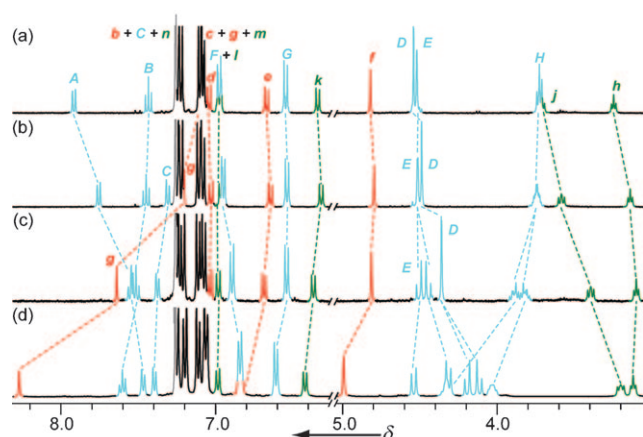
Figure 1. 1 H NMR spectra (400 MHz, CDCl 3 , 300 K) of a) rotaxane 4a , b) rotaxane 4b , c) rotaxane 4c , and d) rotaxane 4d . Labeling as shown in Scheme 1.
