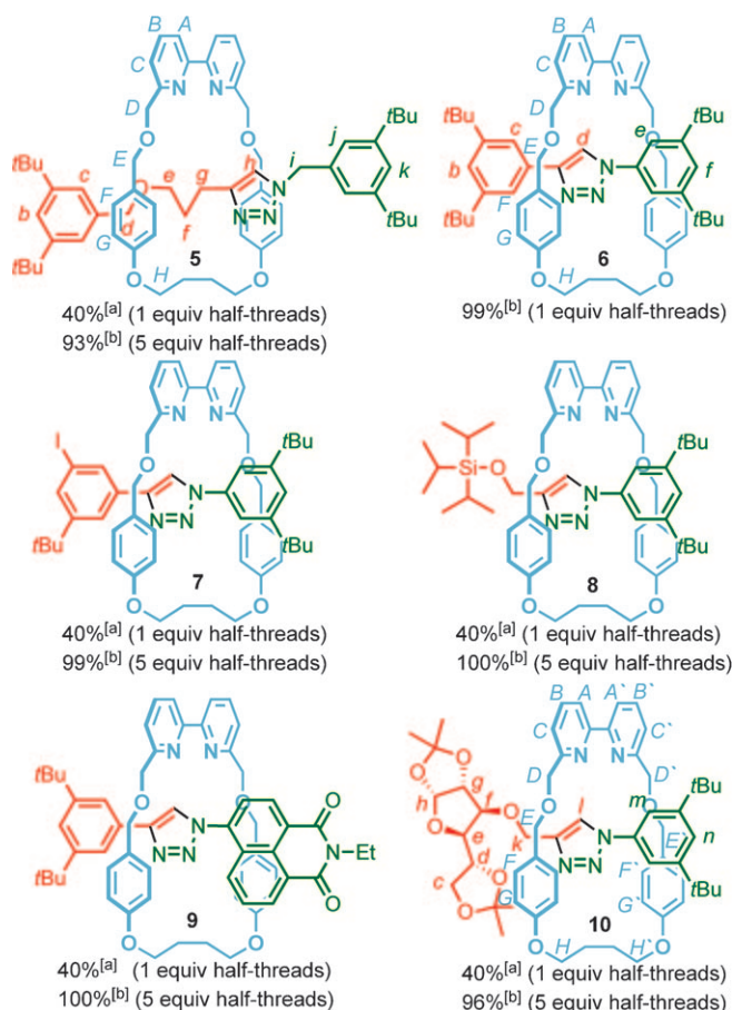
Figure 2. “Small” rotaxanes synthesized using the CuAAC-AT reaction. Reactions were carried out as outlined in Scheme 1 at 80 °C. [a] Determined by 1 H NMR analysis of the crude reaction mixture. [b] Yield of isolated product after column chromatography.
