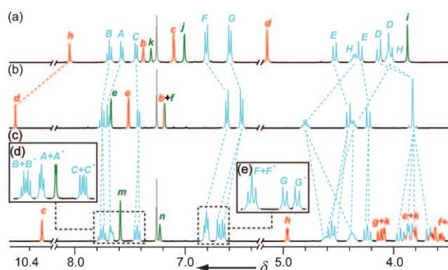
Figure 4. ^1\text{H} NMR spectra (400 MHz, \text{CDCl}_3 , 300 K) of rotaxanes a) 5 , b) 6 , c) 10 , and d) and e) expansions (600 MHz, \text{CDCl}_3 ) of the indicated regions of spectrum (c) demonstrating the rotational dissymmetry of the macrocycle. Labeling as shown in Figure 2.
